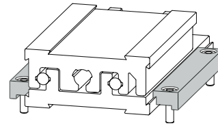
Assembly example
